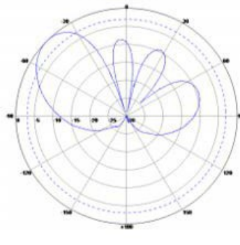
65° Broadcast
