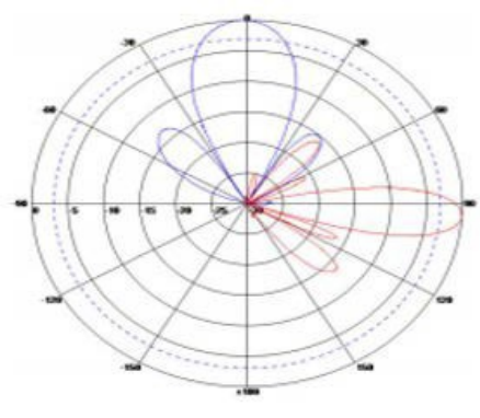
0° Service Beam
