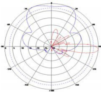
Single Column Beam
